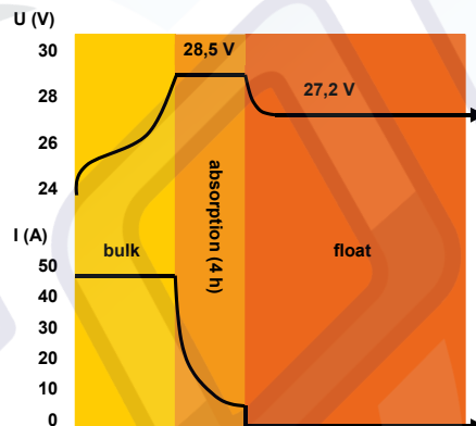
Charge curve
